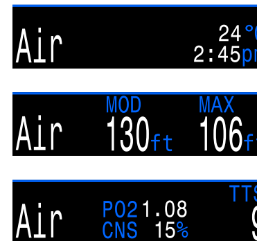
FIGURE 18 Example Configurations for the Bottom Row
